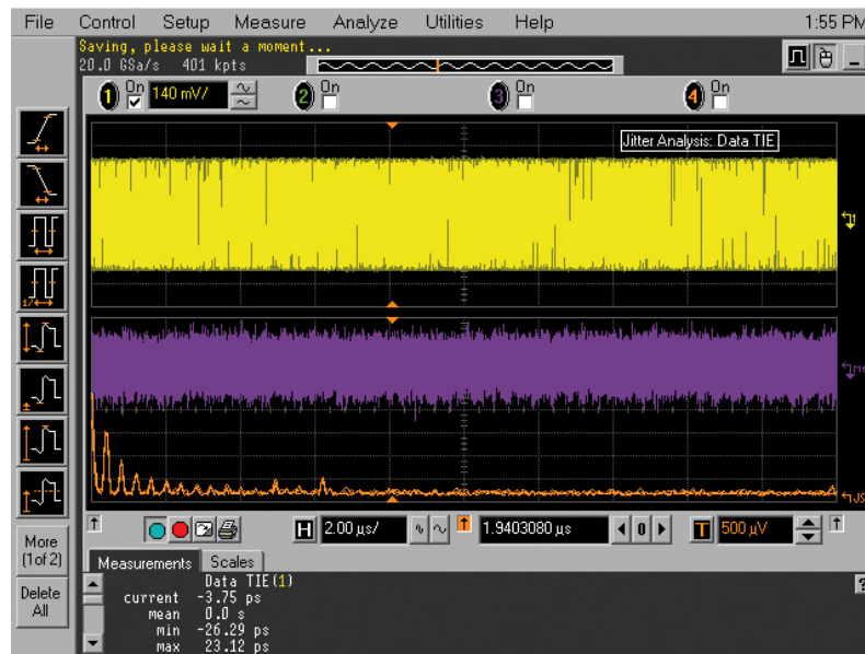
Figure 12: Isolating uncorrelated PJ with a jitter spectrum measurement
