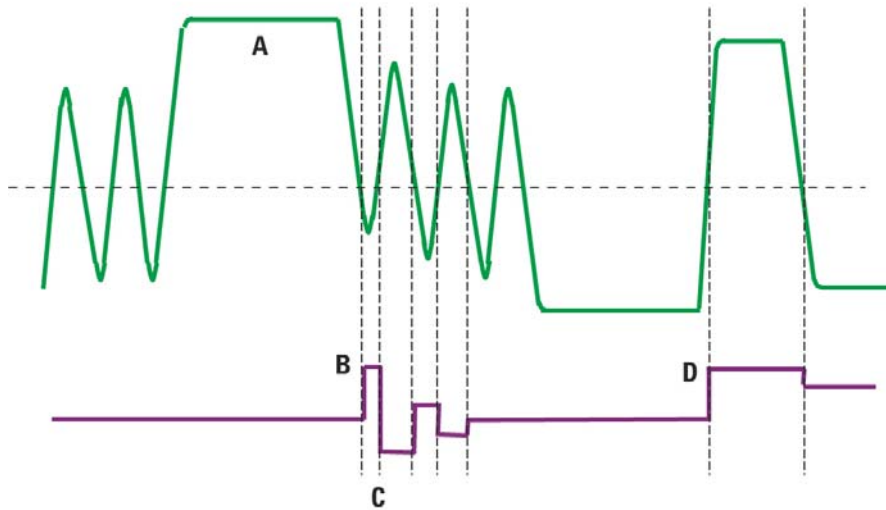
Figure 5: Inter-Symbol Interference (ISI) due to BW Problem
