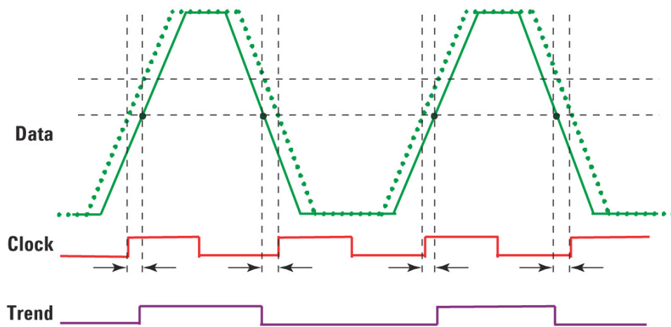
Figure 4: Duty Cycle Distortion (DCD)
