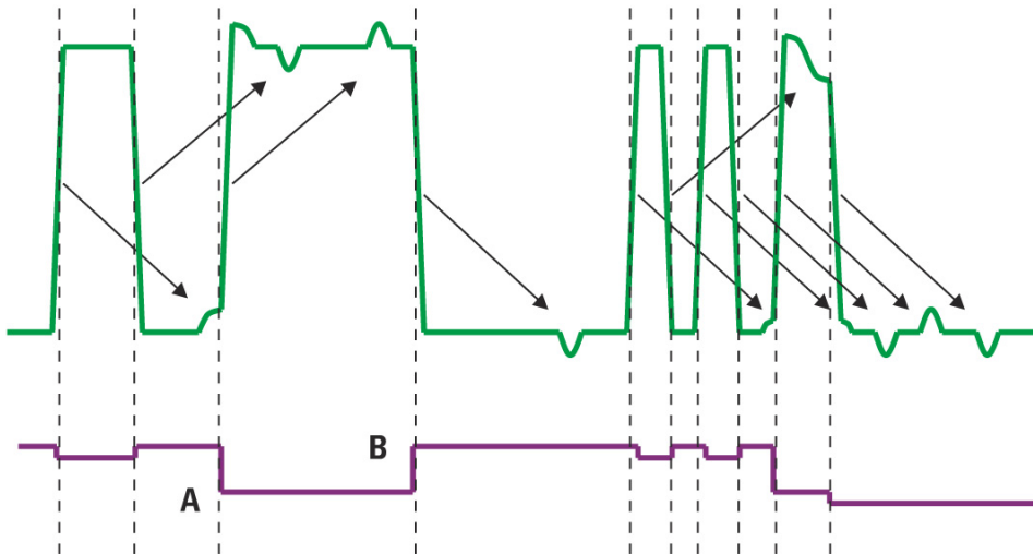
Figure 6: ISI due to reflections
