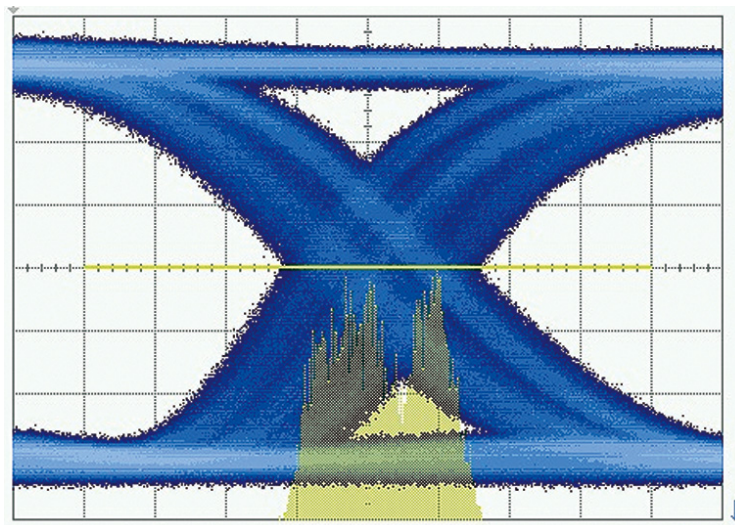
Figure 1: Viewing jitter in an eye-diagram
