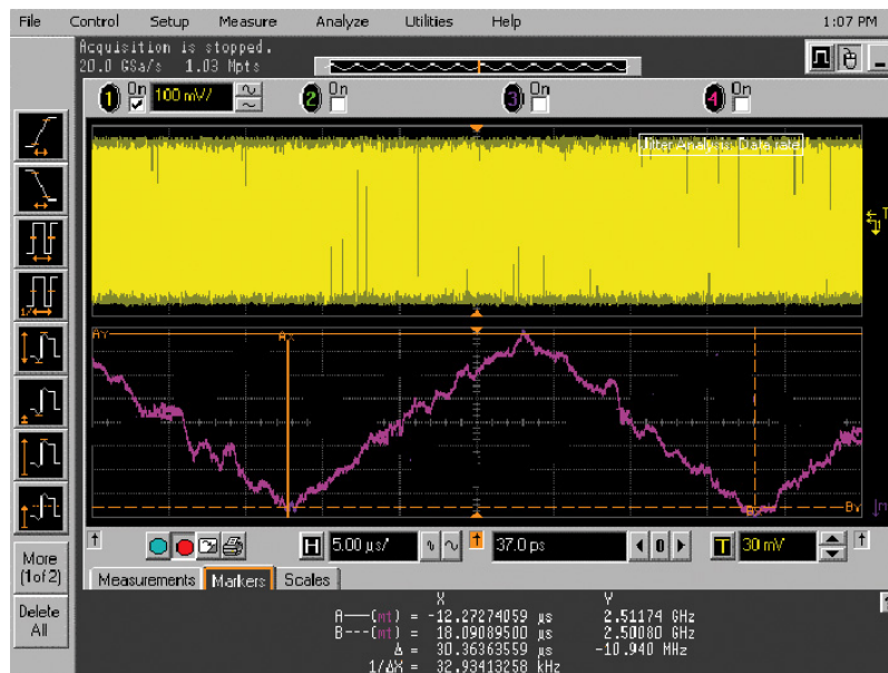
Figure 16: Measuring the Spread Spectrum Clock
