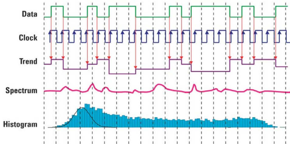
Figure 2: Real-time Jitter Analysis
