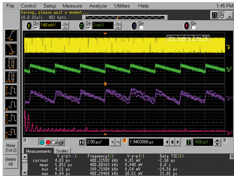
Figure 13: Verifying that switching power supply coupling causes periodic jitter
